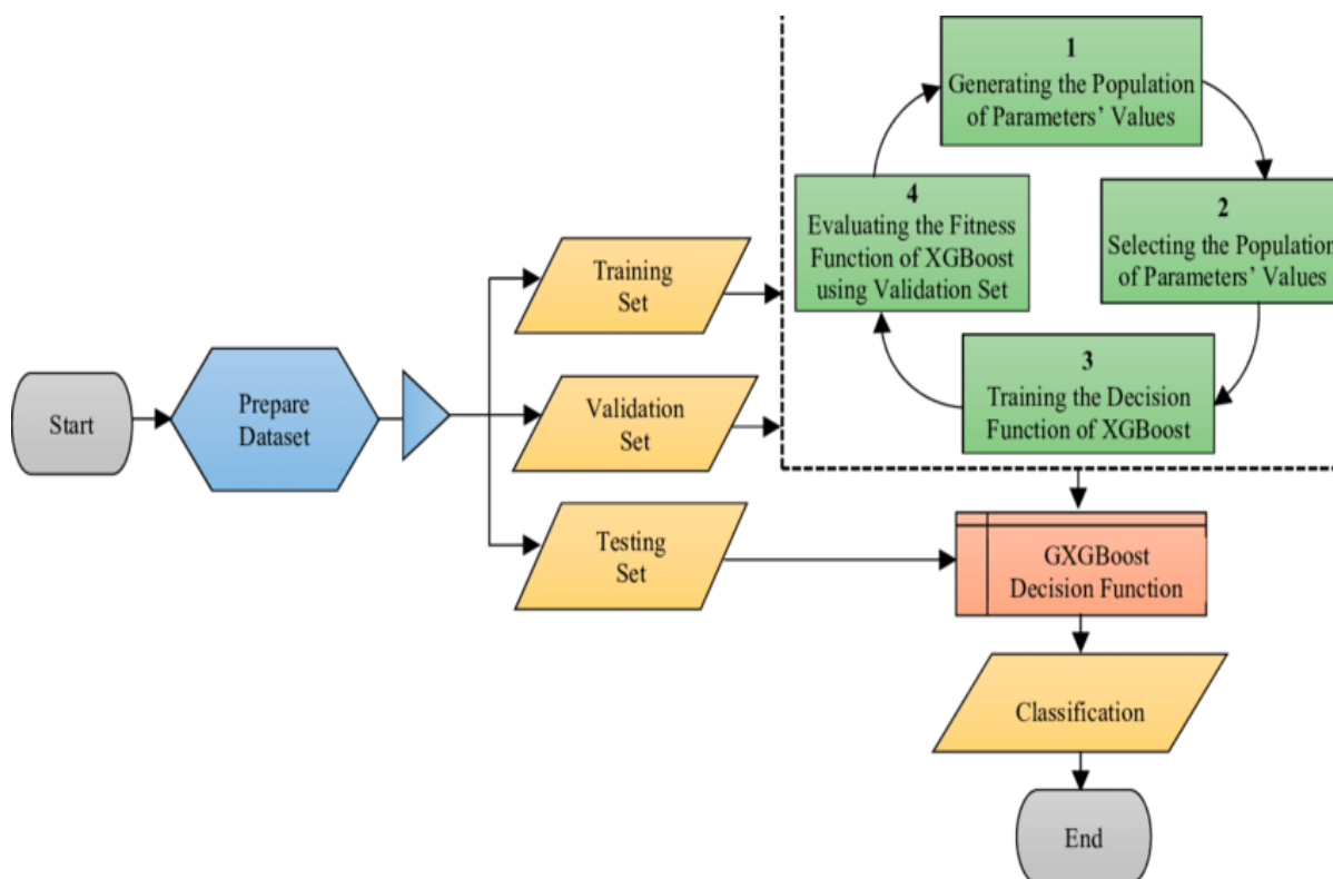
6. Figure 1. XgBoost Algorithm Flowchart
