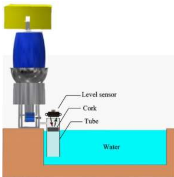
Fig.4.The water level monitoring system
