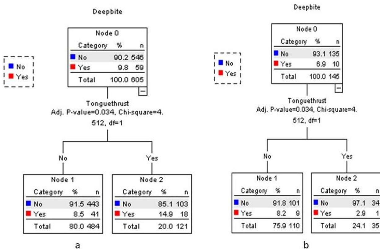
Fig. 4: Decision tree classifier for Deep bite (a) For training data(b) For test data
