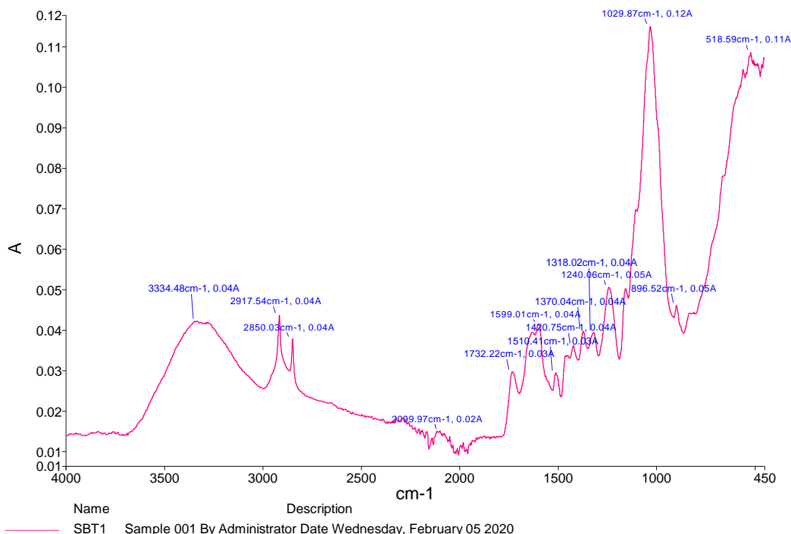
Figure.8. FTIR output
