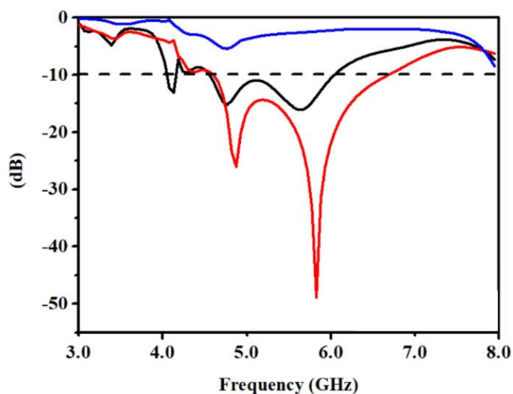
Figure 9: Comparison of simulation with rectangular microstrip array
