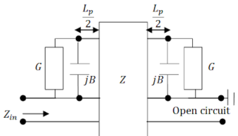
Figure 7: The Circuit model of parallel supply of microstrip
