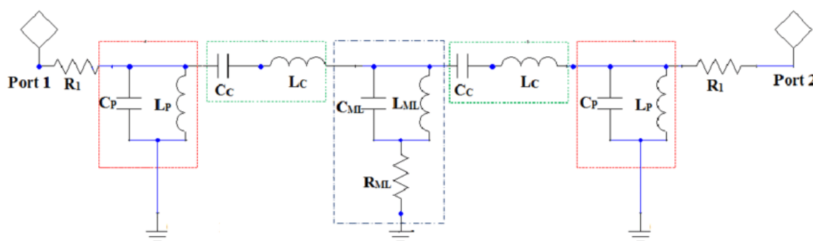
Figure 1: Circuit model for microstrip antennas
