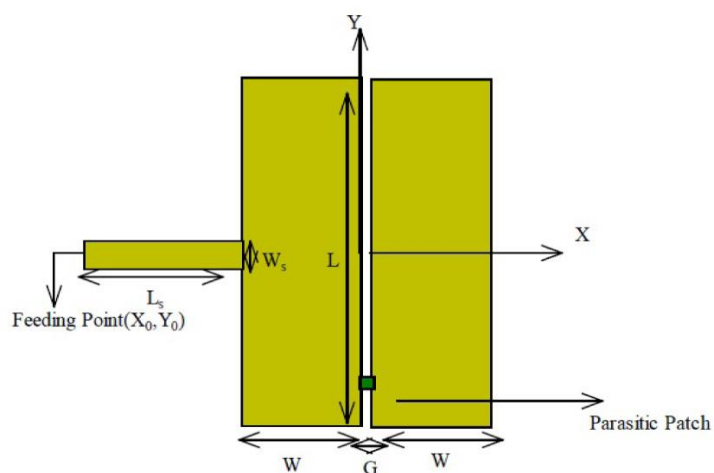
Figure 5: Precise dimensions of the microstrip patch array supplied in series
