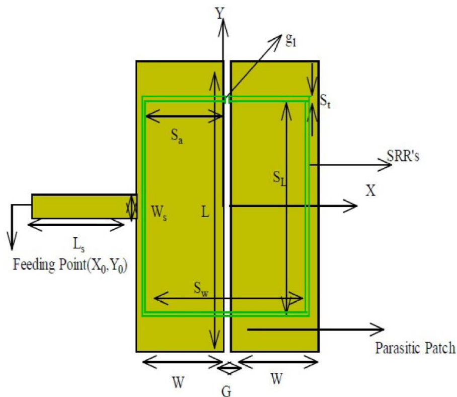
Figure 3: Microstrip patch array dimensions in detail
