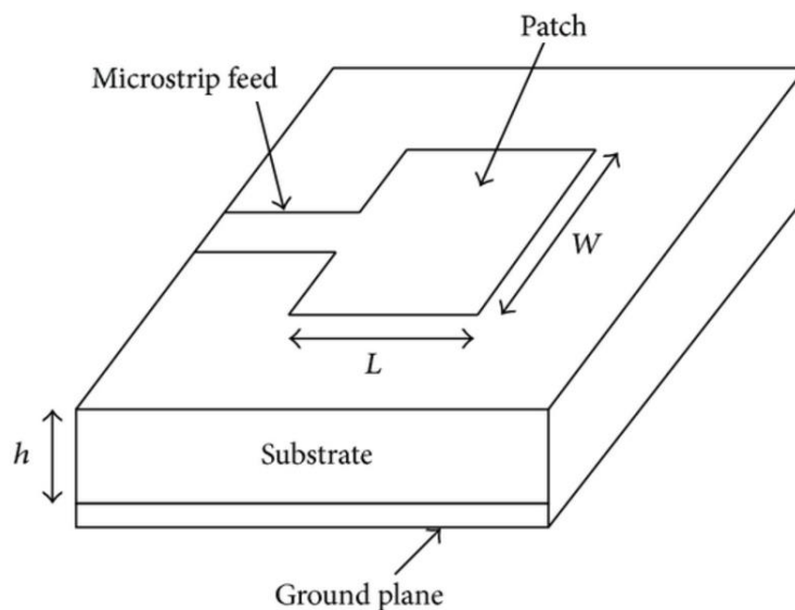
Figure 2: A three-dimensional image of a rectangular microstrip array
