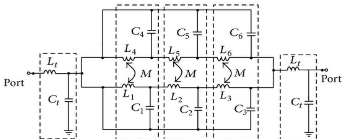
Figure 4 presents the full comparable Circuit Model of the planned business rectangular microstrip arrangement Q11 with all applications.
