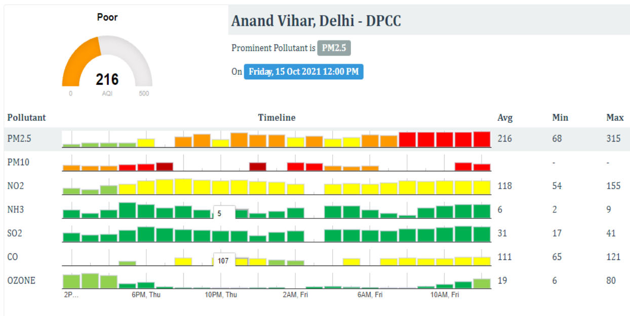
Fig.2 Pollutants average values of Delhi on a specific Day
