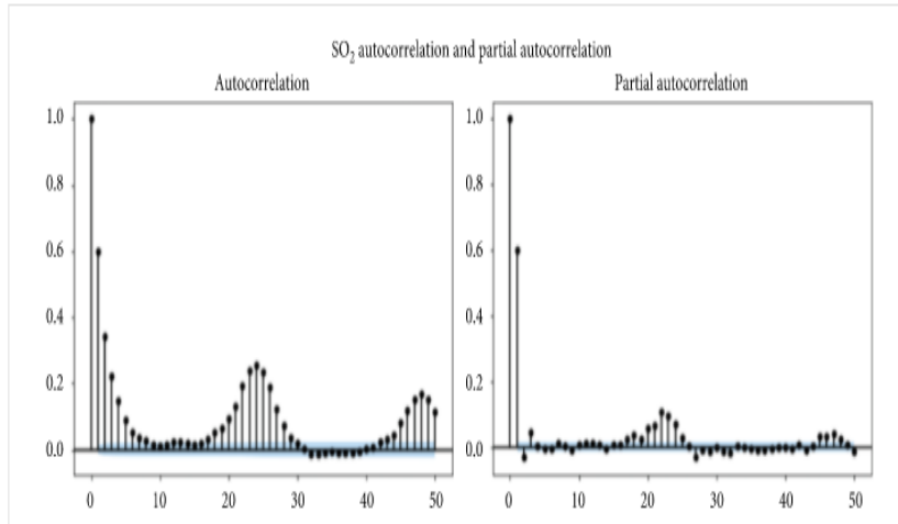
Fig 5: Partial Autocorrelation
