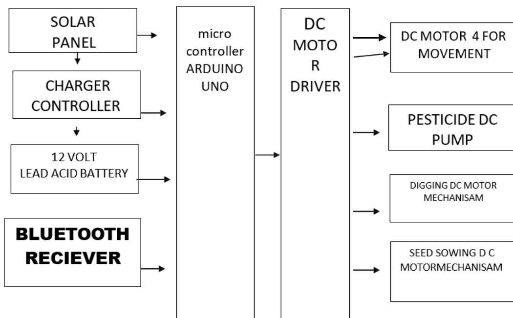
Figure.9. Layout of the Receiver
